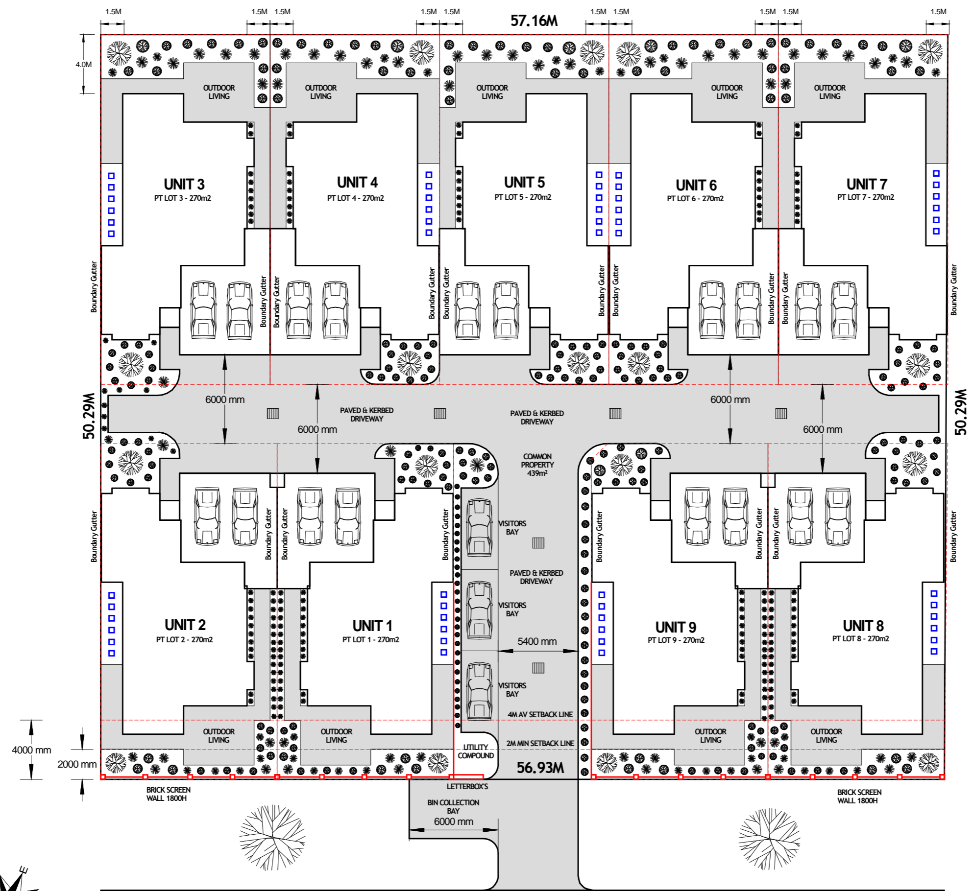
SITE PLAN 1:250 - (PRELIMINARY)
